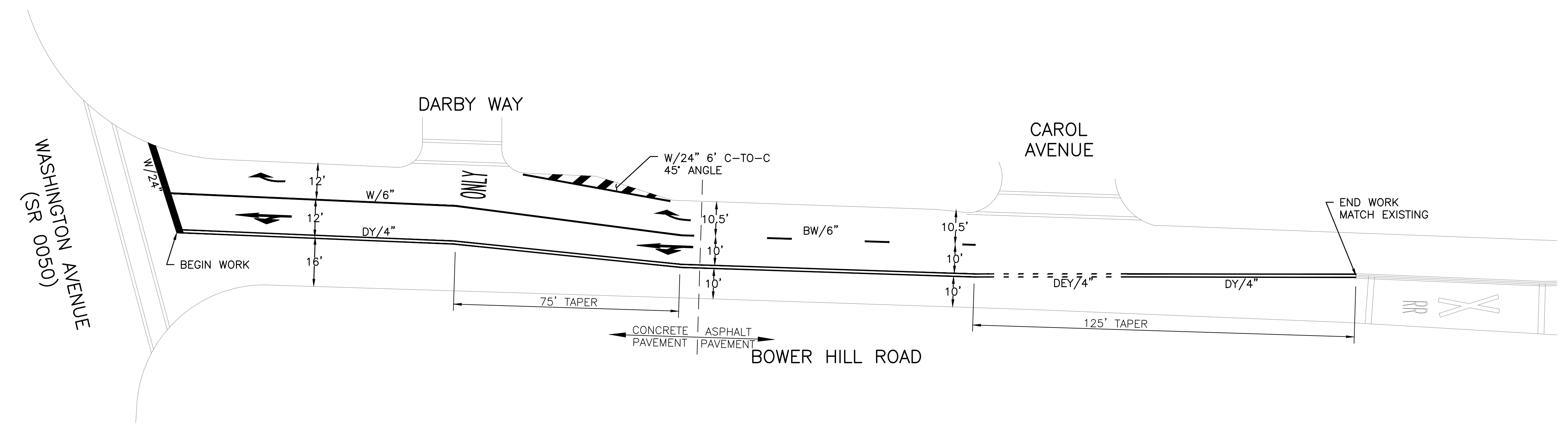
PROPOSED CONDITIONS PLAN
